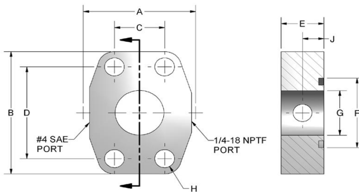
GAGE PORT SPACER-CODE 62
