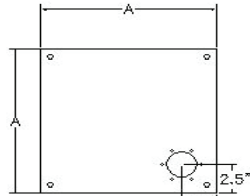
TVL-934A c/w Filler Cutout
