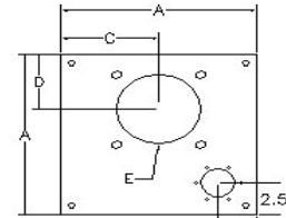
TVL-940A c/w Filler Cutout Motor Adaptor Cutout Adaptor Style 7
