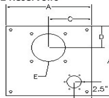
TVL-926 c/w Filler Cutout Motor Adaptor Cutout adaptor Style 1,1A,1B
