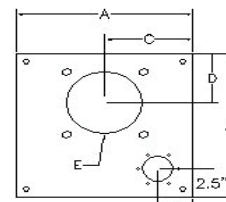
TVL-929A c/w Filler Cutout Motor Adaptor Cutout Adaptor Style 7
