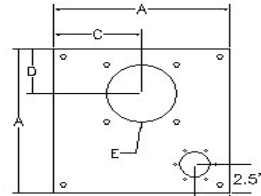
TVL-937A c/w Filler Cutout Motor Adaptor Cutout Adaptor Style 1
