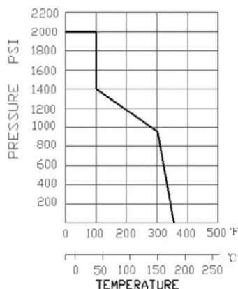
PRESSURE-TEMPERATURE RATING
